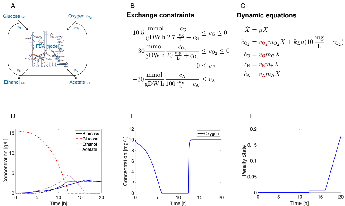
Figure 10.4: Example result of a dFBA simulation for the E. coli core model [97] performed with DFBAlab. (A) Illustration of dynamic metabolites and relevant exchange fluxes. Extracellular metabolites use mass concentration (g/L), exchange fluxes are in molar amount per dry biomass and time (mmol/gDW h). (B) Concentration-dependent constraints applied to the exchange fluxes during the dFBA simulation. (C) Differential equation model for biomass concentration X and metabolite mass concentrations. Growth rate \mu and exchange fluxes v_* (in red) are optimal values from the underlying FBA model. m_{O_2} , m_G , m_E , m_A are molar masses of O_2 , glucose, ethanol, and acetate, respectively. k_L a = 8.5 \text{ h}^{-1} is the volumetric mass transfer coefficient for oxygen. (D) Simulation results for concentrations of biomass and metabolites. We can observe four growth phases: aerobic growth on glucose with production of acetate, anaerobic growth on glucose with production of ethanol and acetate, aerobic growth on acetate, and a stationary phase. (E) Simulation result for oxygen concentration in the liquid medium. Oxygen is depleted in the second growth phase due to mass transfer limitations, but replenishes at the start of the third phase. (F) Penalty function time course. Increases of the penalty function indicate periods where the underlying FBA model is infeasible. Here, this occurs when the ATP maintenance constraint cannot be satisfied due to a lack of substrates, and happens in this simulation during a brief period where the switch from glucose to acetate as a substrate takes place, since oxygen needs to be replenished first, and in the stationary phase.
